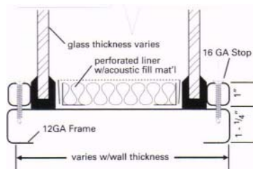
"HM" Frame Design
