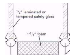
"U" Frame Design
