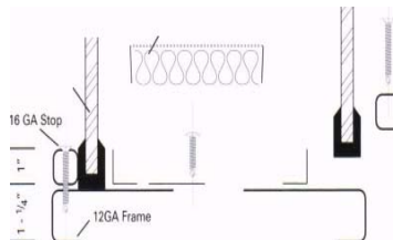
"Split-Frame" Design
